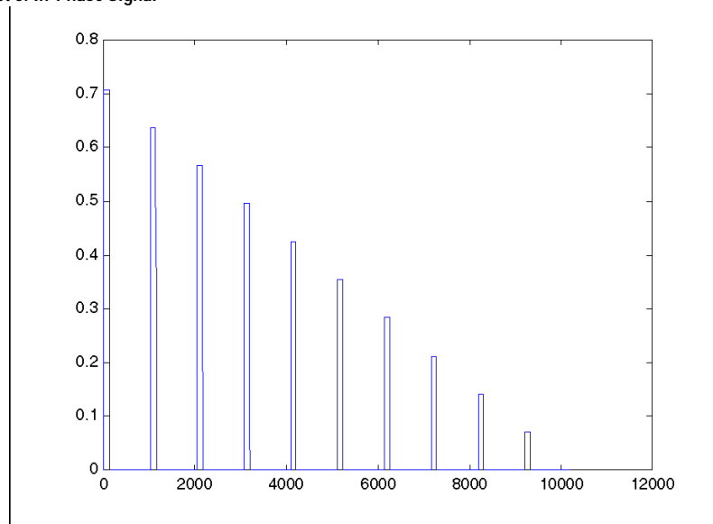
Figure 11 Simulated Plot of In-Phase Signal
